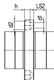
Pilot Flange Type
